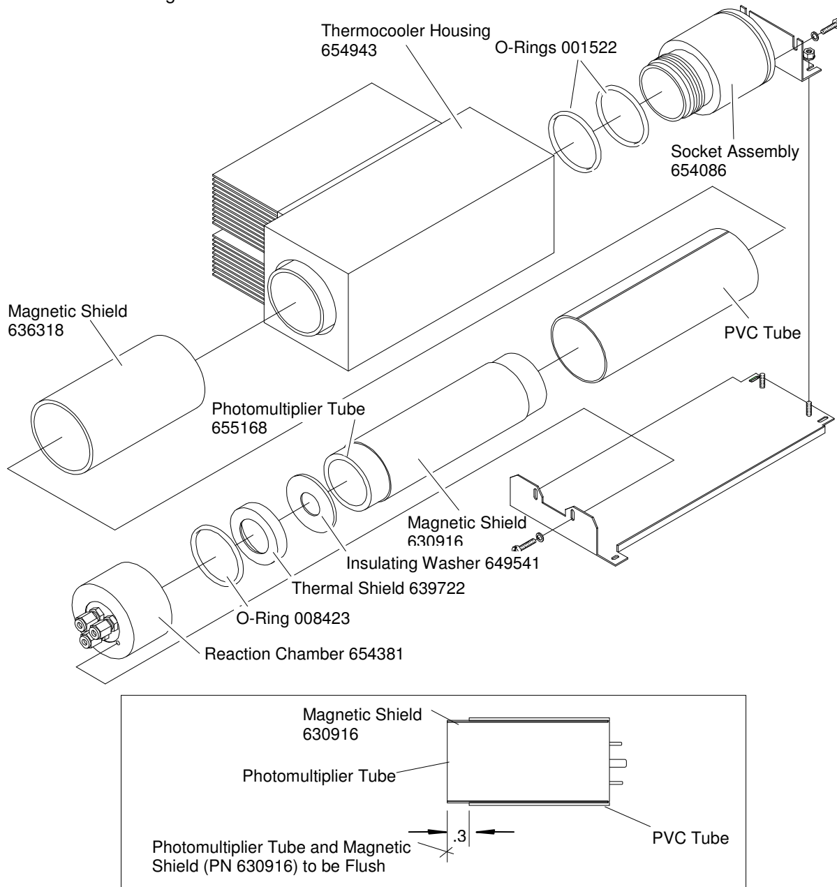
Figure 6-2. Photomultiplier Housing Assembly
